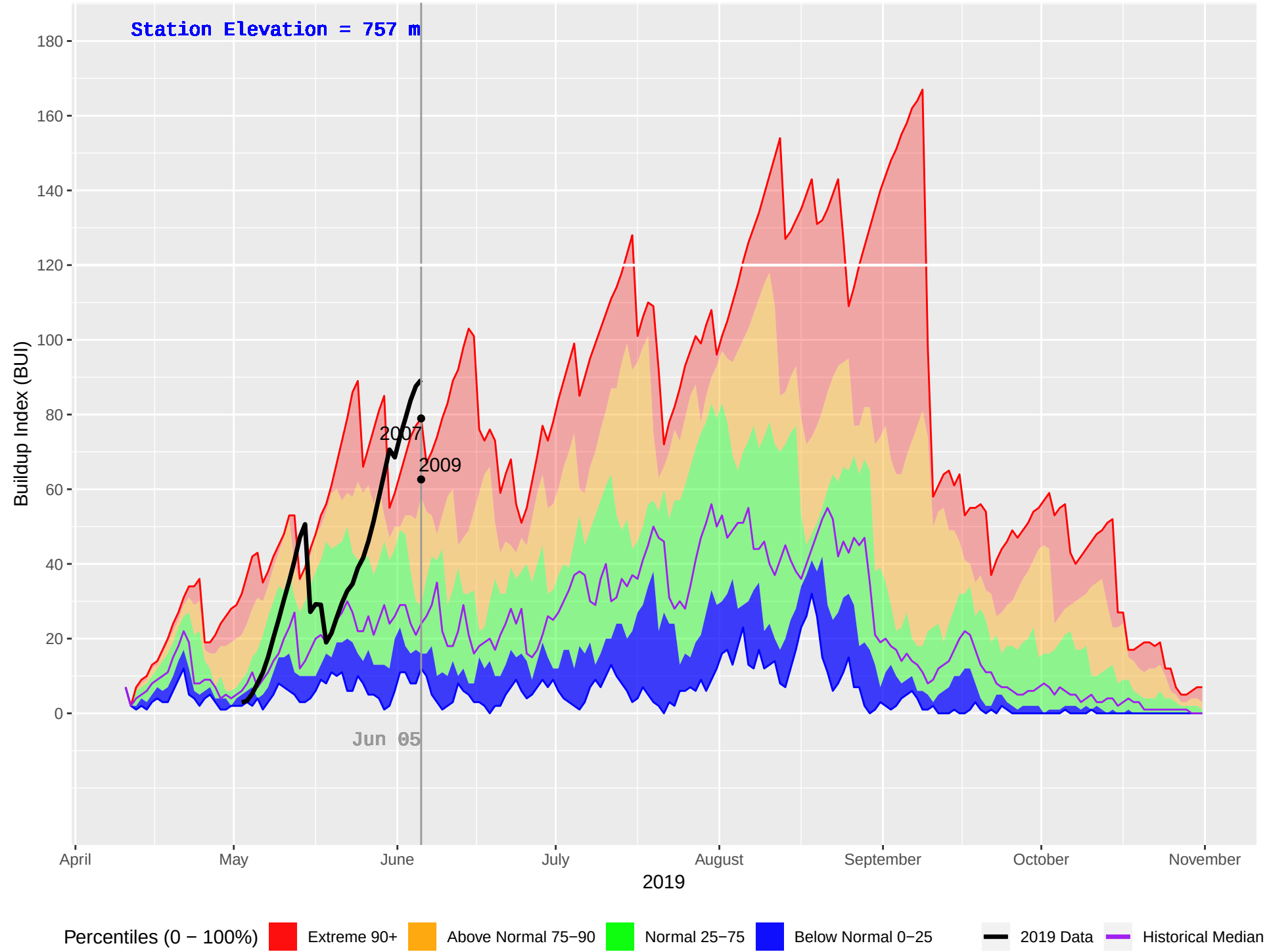
DOWNIE (905) : Historical (2005–2018), Current (2019) Daily Buildup Index (BUI)
