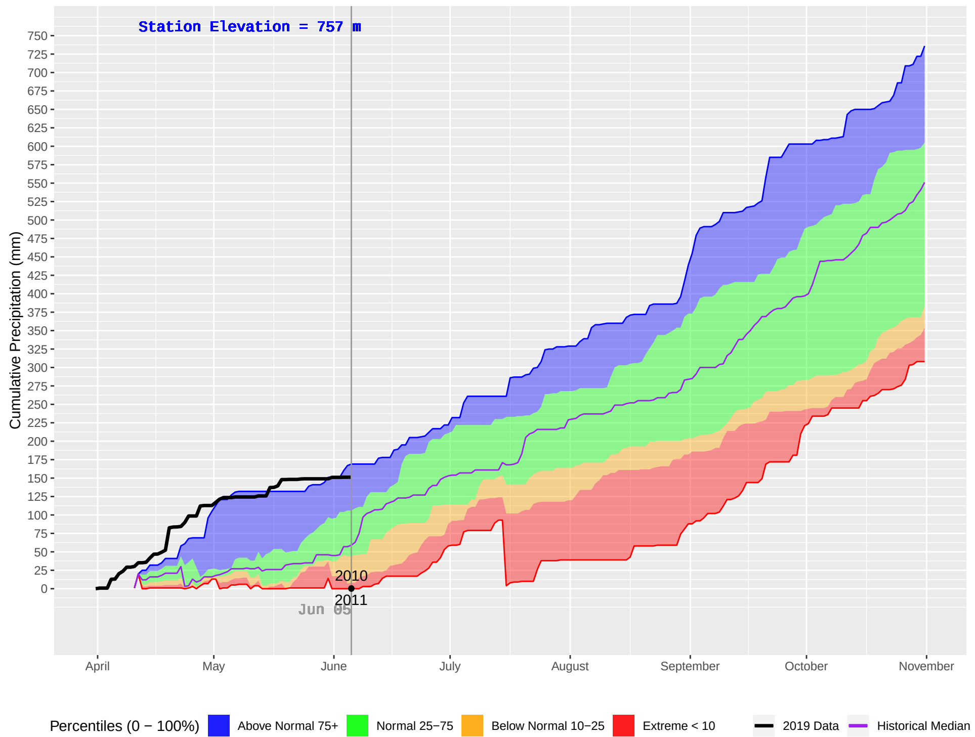
DOWNIE (905) : Historical (2005–2018), Current (2019) Daily Cumulative Precipitation
