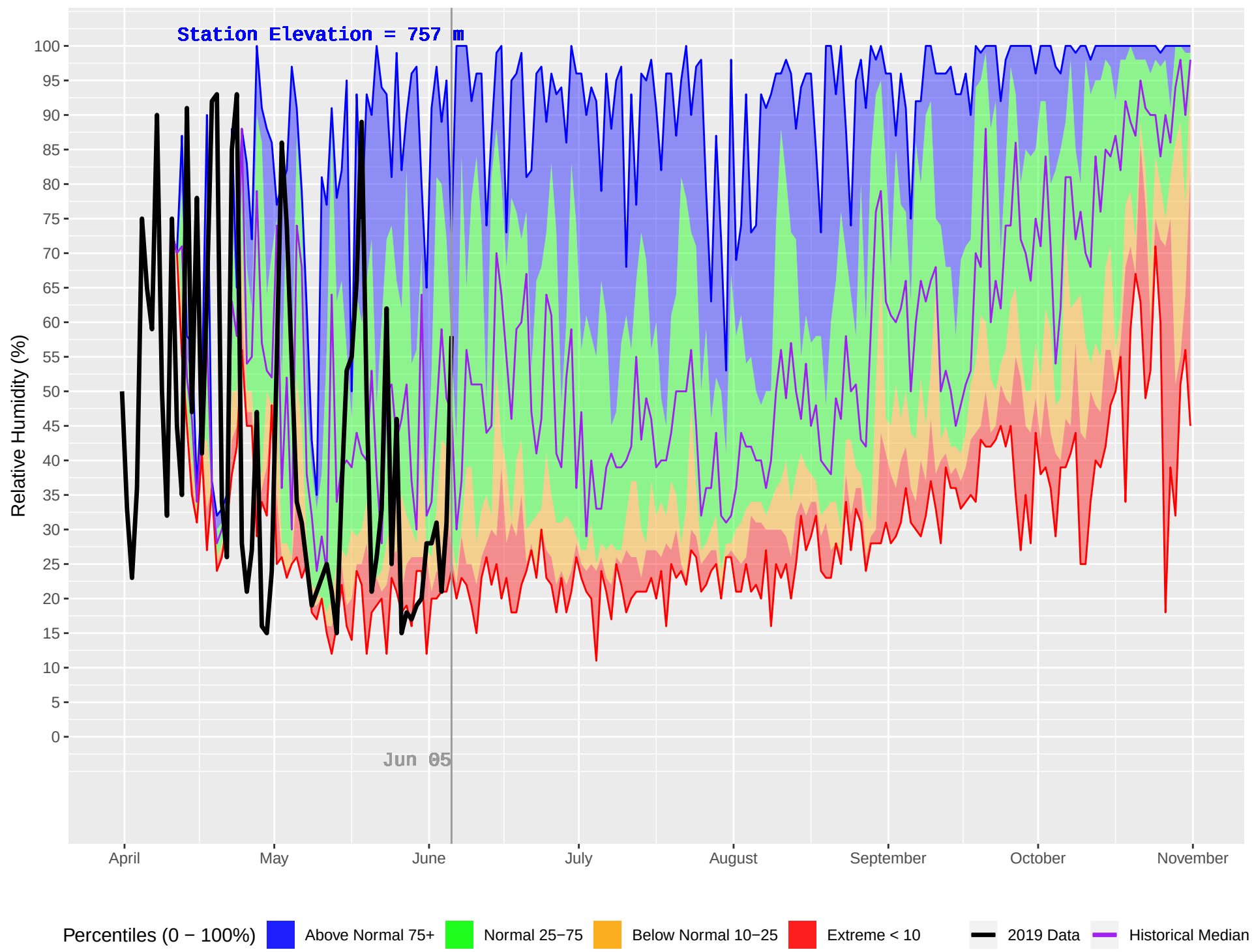
DOWNIE (905) : Historical (2005–2018) and Current (2019) Daily Relative Humidity
