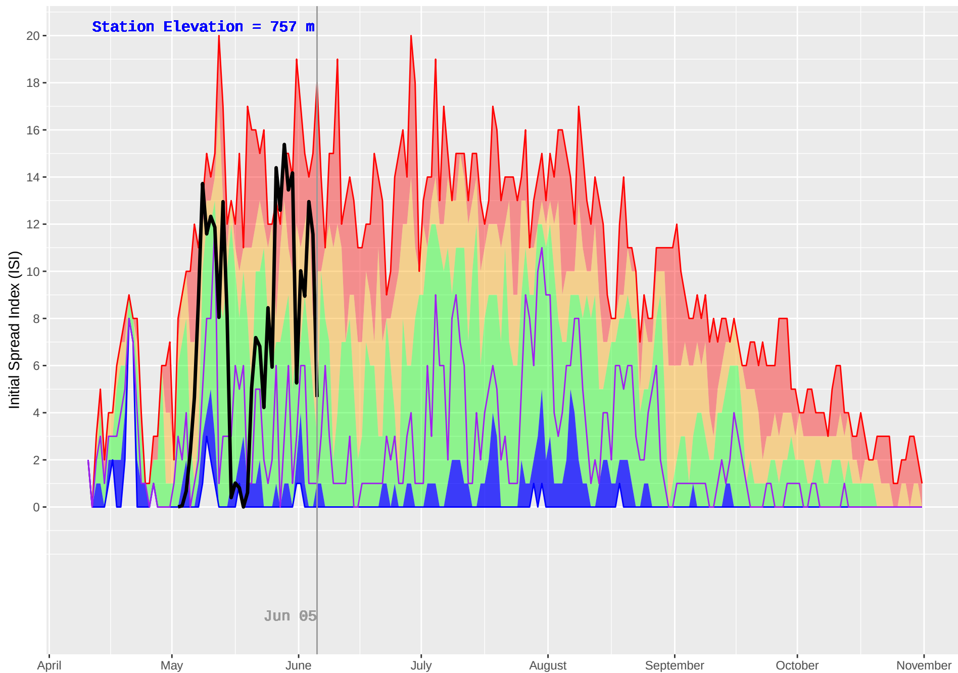
DOWNIE (905) : Historical (2005–2018) and Current (2019) Daily Initial Spread Index (ISI)
