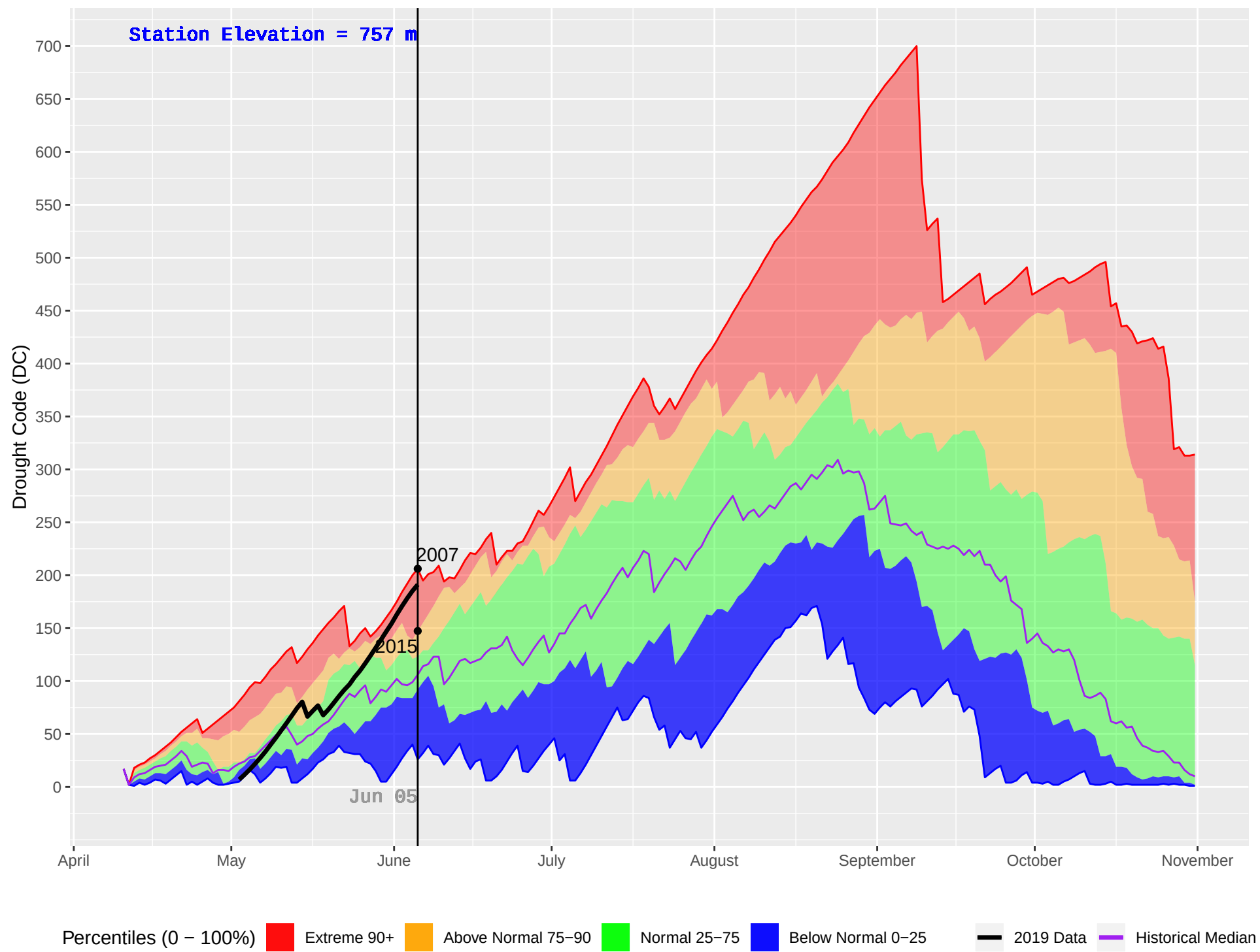
DOWNIE (905) : Historical (2005–2018) and Current (2019) Daily Drought Code (DC)
