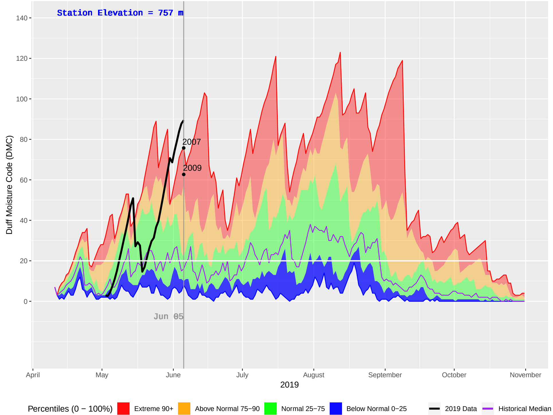
DOWNIE (905) : Historical (2005–2018), Current (2019) Daily Duff Moisture Code (DMC)
