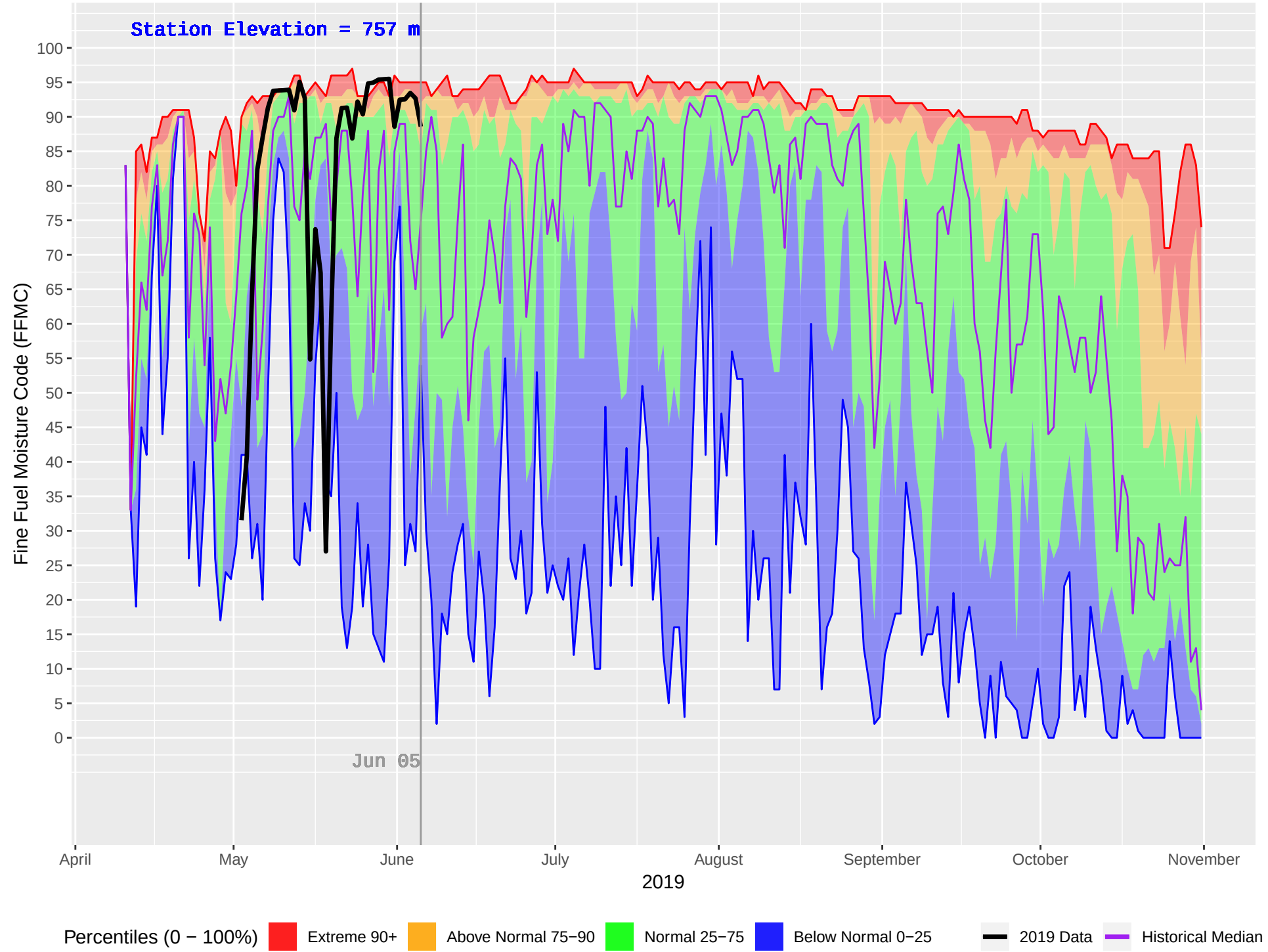
DOWNIE (905) : Historical (2005–2018) and Current (2019) Daily Fine Fuel Moisture Code (FFMC)
