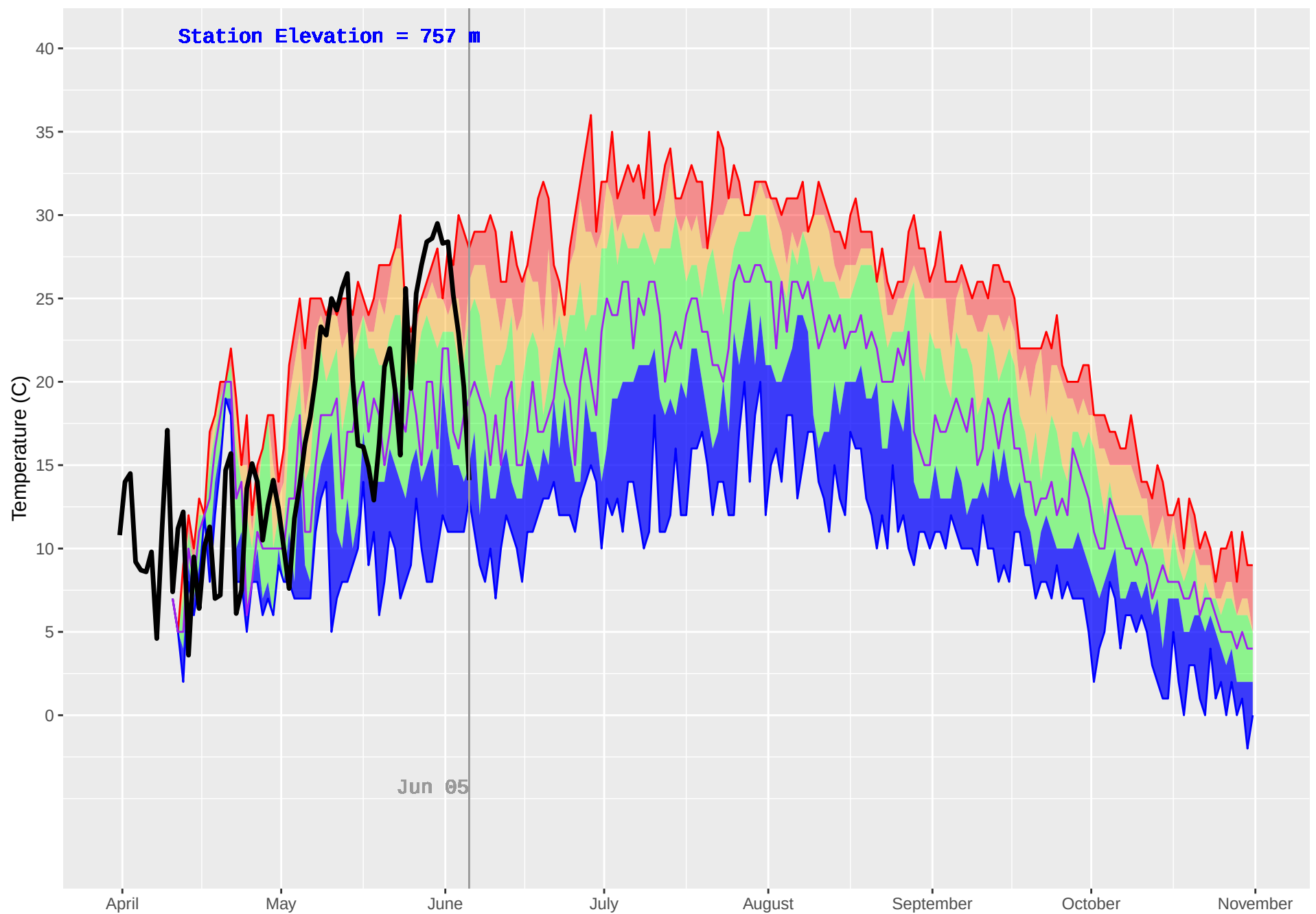
DOWNIE (905) : Historical (2005–2018) and Current (2019) Daily Temperature
